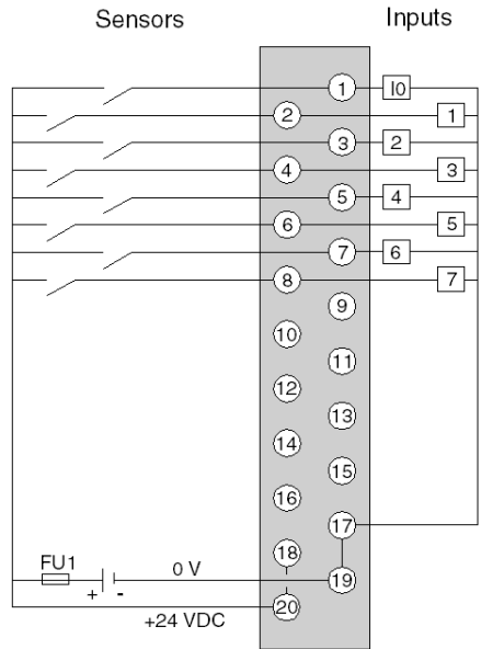
FU1 0.5 A quick-blow fuse
