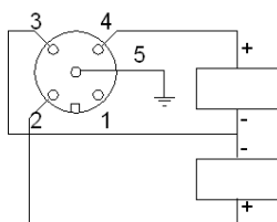
Direct wiring
