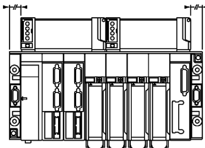
8 position racks (TSX RKY 8/8EX)
