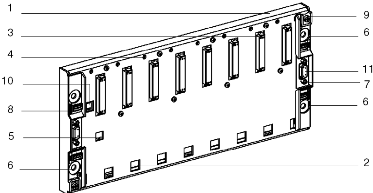
Extendable rack
