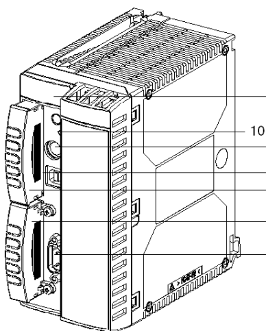
Double format processor: TSX P57 554
