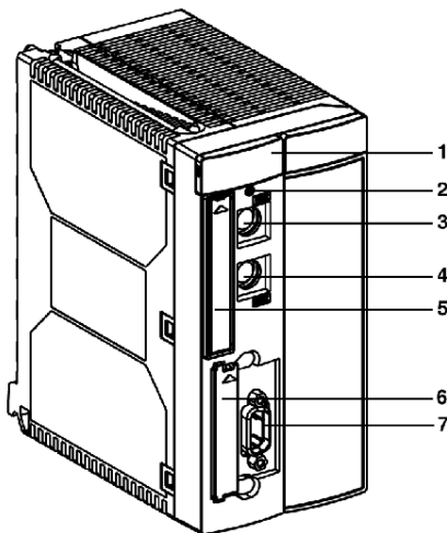
Double format processor: TSX P57 204/254/304/354/454
