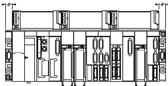
12 position racks (TSX RKY 12/12EX)
