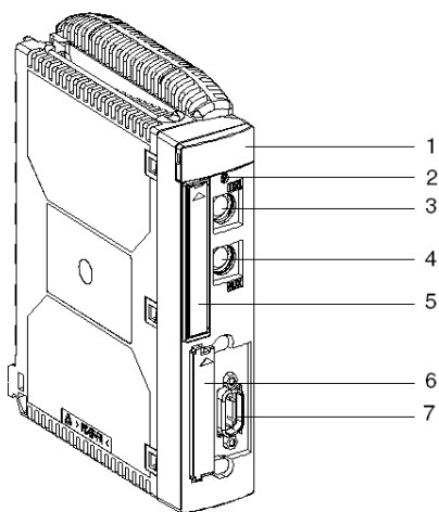
Standard format processor: TSX P57 0244/104/154
