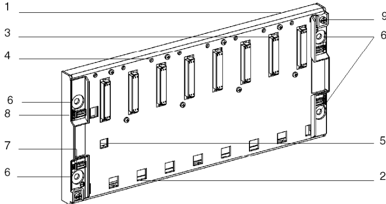
Standard rack
