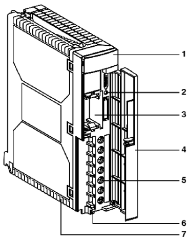
Standard format
