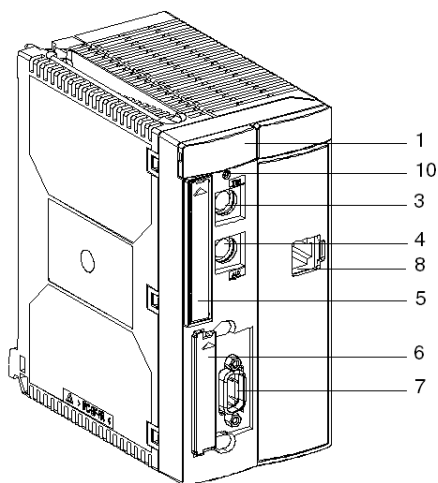
Double format processor: TSX P57 1634/2634/3634/4634
