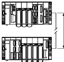
Station with extendable racks: 2 racks 12 positions or 4 racks 4, 6 or 8 positions, maximum length of X-Bus: 100 meters
