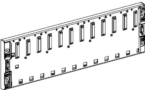
TSX RKY extendable rack (12 positions)
