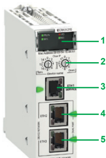
BMECRA31210
