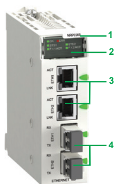
BMXNRP020●
