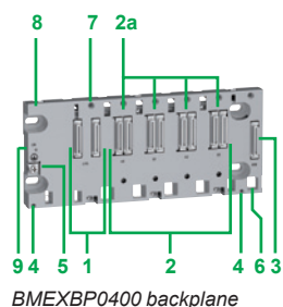
BMEXBP0400 backplane
