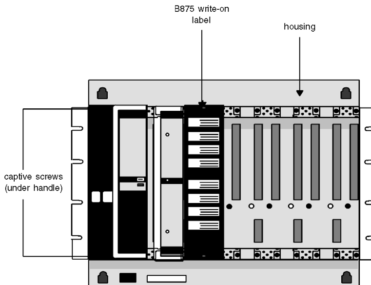
Write-on label plate placement, diagram
