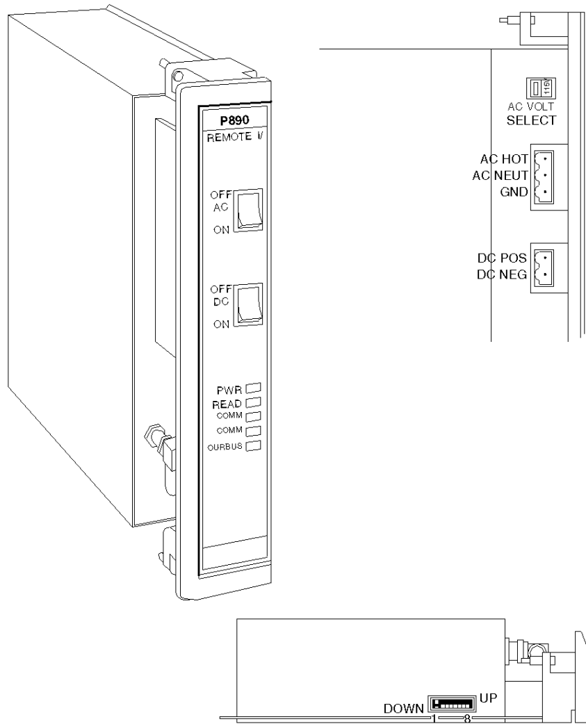
Front, bottom and side view
