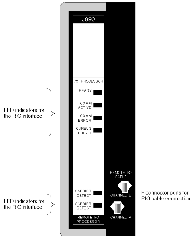
AS-J890 front view
