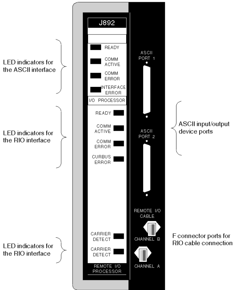
J892 front view
