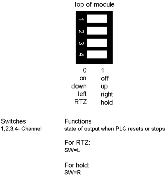
4- Position DIP- Switches
