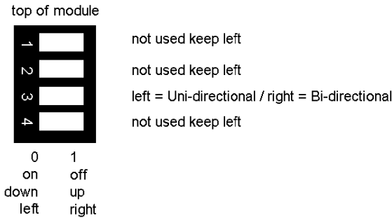
4- position DIP switches
