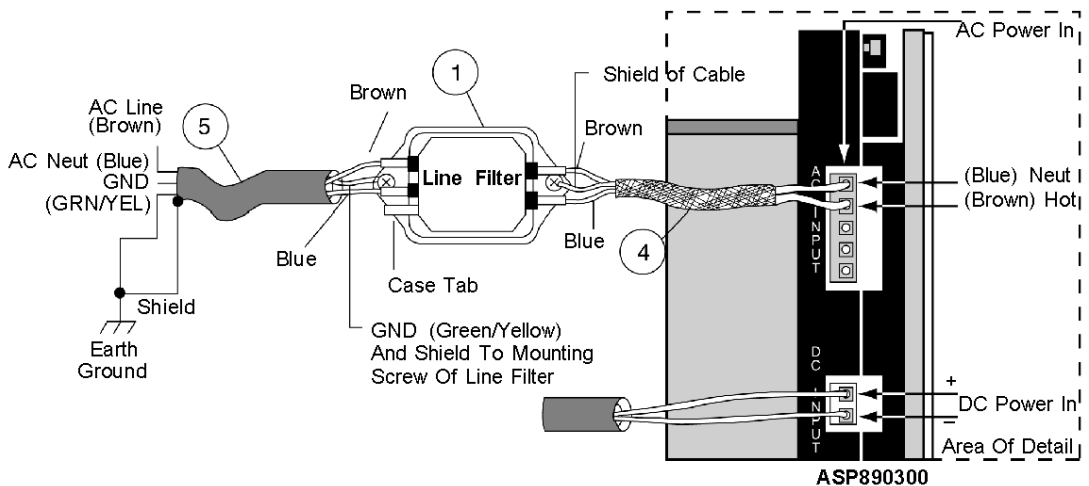
Typical CE Installation for a Remote Drop
