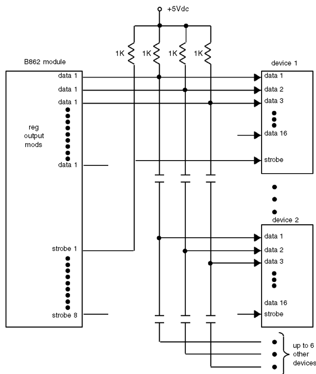
Pull-up Resistor Connection
