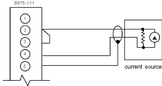
Field connector jumper diagram
