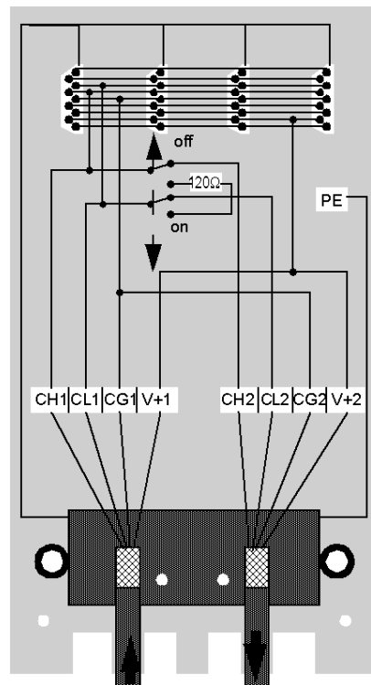
Cable preparation template
