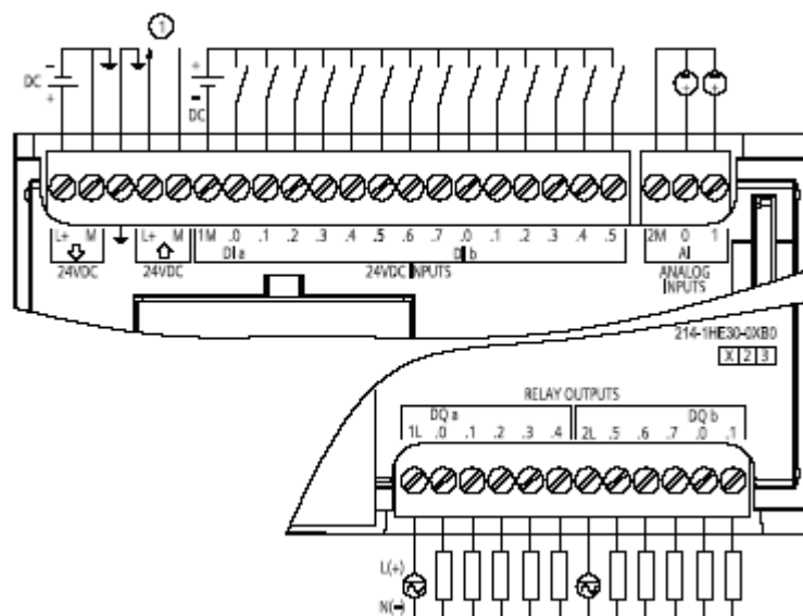
Рис. A-8. CPU 1214C DC/DC/Relay (6ES7 214-1HE30-0XB0)
