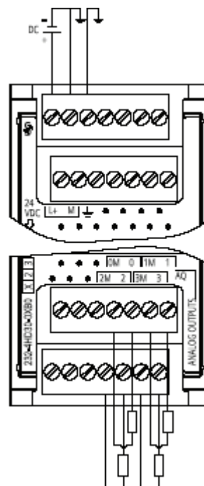
SM 1232 AQ 4 x 14 Bit
