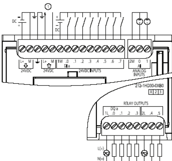
Рис. A-5. CPU 1212C DC/DC/Relay (6ES7 212-1HD30-0XB0)
